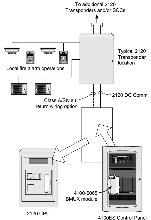
2120 CPU Replaced with 4100ES Control Panel
