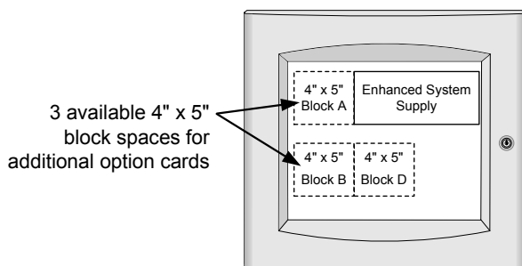
Mounting Locations for Optional Modules, One-Bay Cabinet
